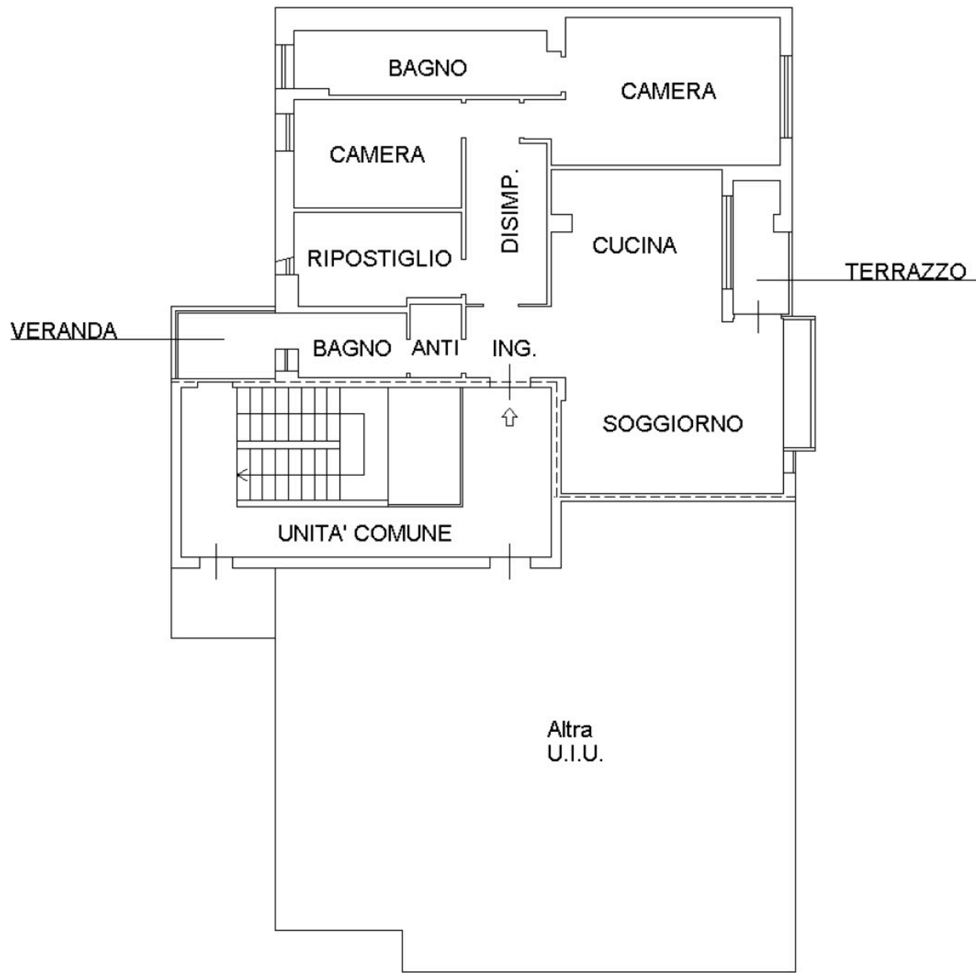
PIANTA PIANO QUINTO H = 2,70 m
